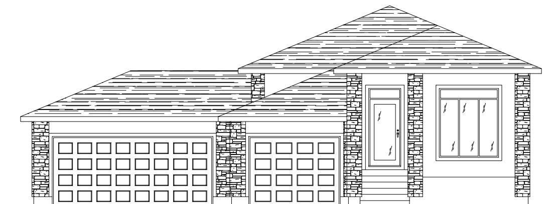
—FRONT ELEVATION—
